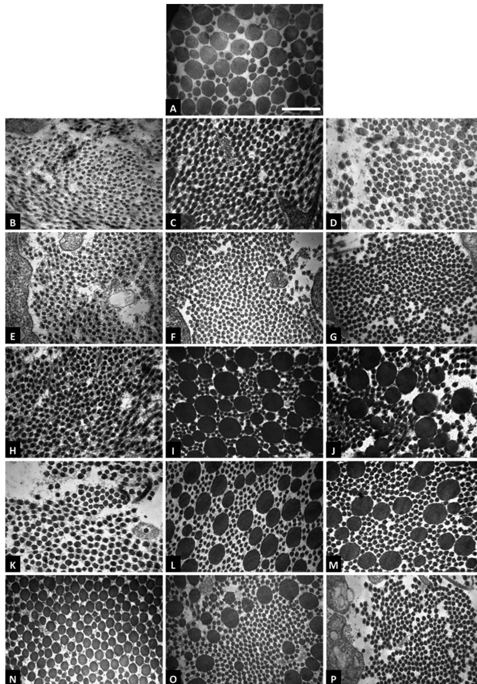
Figure 1 Electron micrographs demonstrating collagen fibril diameters in the different experimental groups (n=4 each): normal (A); tenotomised at day 7 (B), day 14 (C) and day 21 (D) after injury; manual acupuncture at ST36 at day 7 (E), day 14 (F) and day 21 (G); manual acupuncture at BL57 at day 7 (H), day 14 (I) and day 21 (J); manual acupuncture at ST36+BL57 at day 7 (K), day 14 (L) and day 21 (M); and electroacupuncture at ST36+BL57 at day 7 (N), day 14 (O) and day 21 (P). A mixture of large and thin fibrils is apparent in the normal group. After injury, the collagen fibril diameters decreased in the tenotomised and ST36 groups. Large fibrils were present in the BL57 and ST36+BL57 groups at days 14 and 21 and in the electroacupuncture group at day 14. By contrast, these large fibrils were not seen in the electroacupuncture group at day 21. Bar=500 nm.
