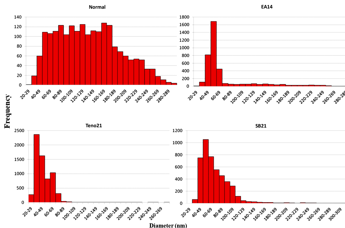
Figure 2 The frequency distributions of collagen fibril diameters in selected experimental groups: normal, tenotomised only at day 21 (teno21), electroacupuncture at ST36+BL57 at day 14 (EA14) and manual acupuncture at ST36+BL57 at day 21 (SB21) after injury. In the groups with injury there was an increase in the frequency of thin (30–69 nm) collagen fibrils. The frequency of thick fibrils (100–259 nm) was increased in the EA14 group and SB21 groups. The reorganisation of collagen fibril diameters was improved in the EA14 group—the values did not differ statistically from those of the normal (non-tenotomised) group.
